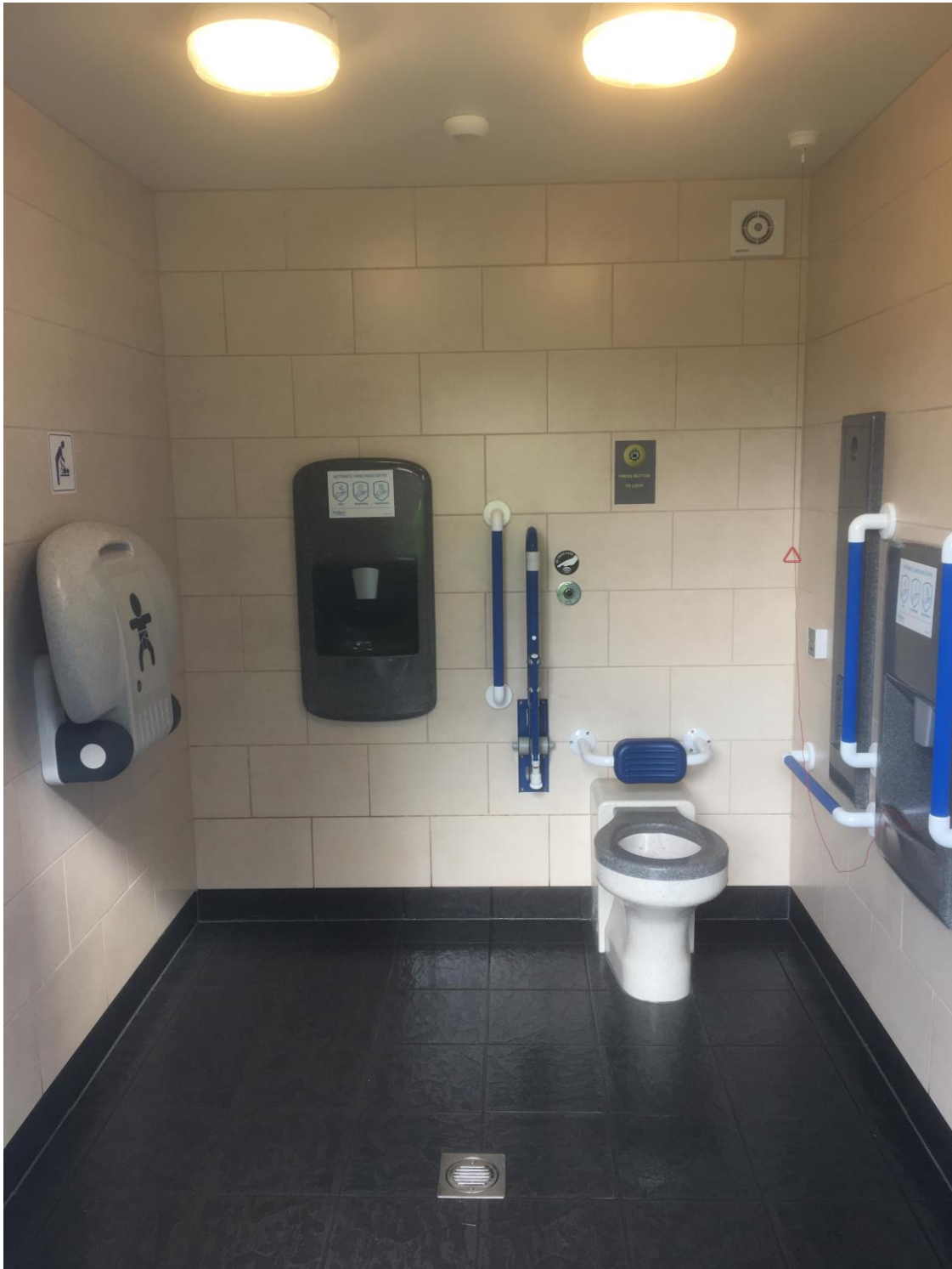
Typical Interior of a disabled accessible cubicle
